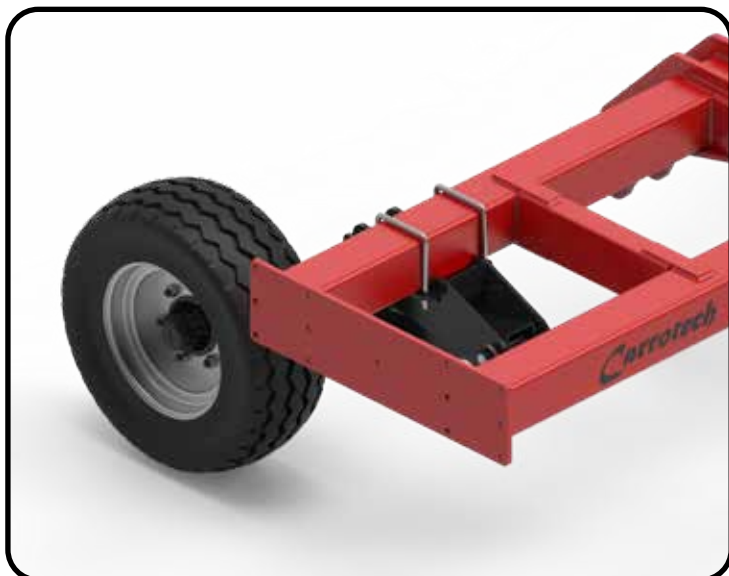
Front Mounted Depth Wheel
