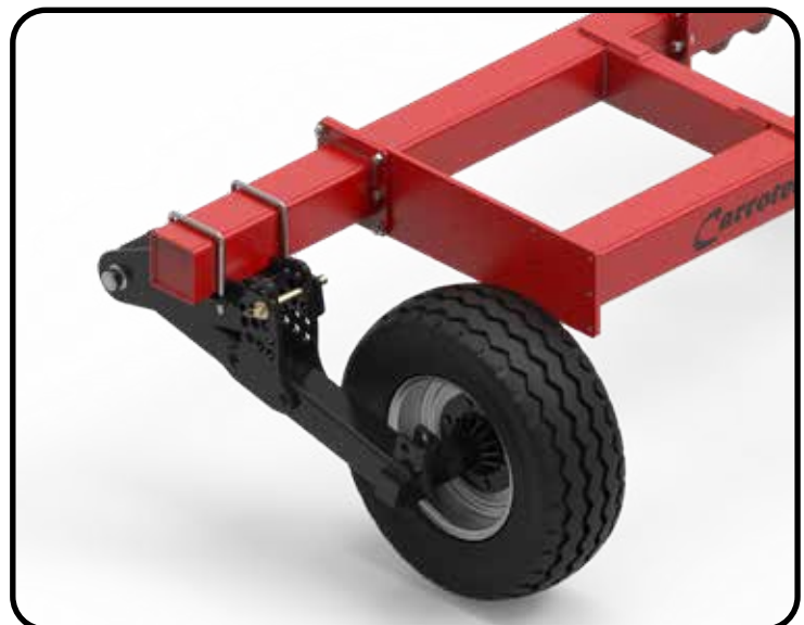
Rear Mounted Depth Wheel
